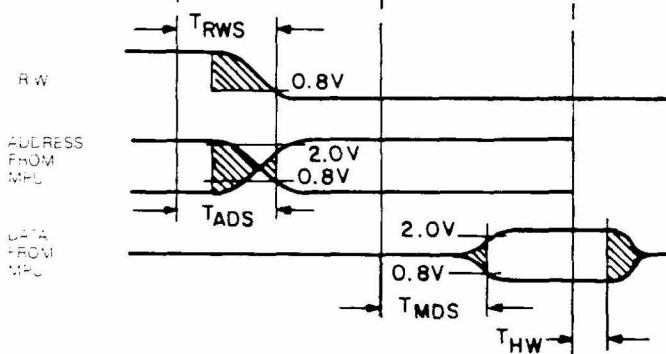
Timing for Writing Data to Memory or Peripherals
