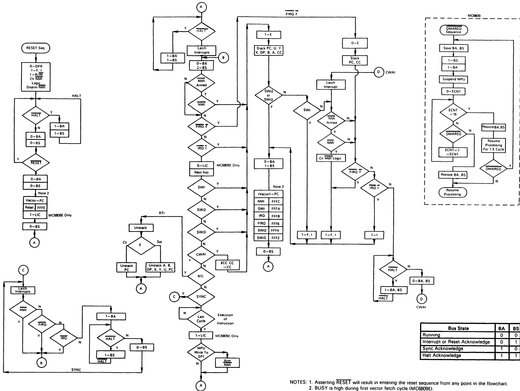
Figure 3-1. Interrupt Processing Flowchart
