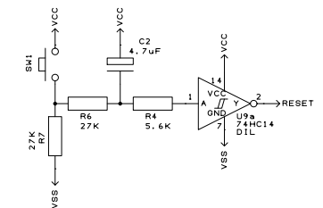
Reset circuit
