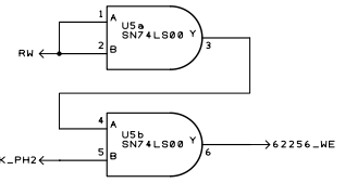
Write RAM on PH2 clock
