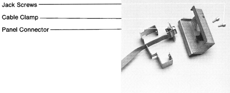
Figure 2-6. Attaching the Cable to the Cable Clamp
