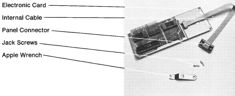
Figure 2-1. Apple IIe Connector Parts
