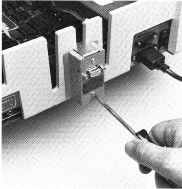
Figure 2-9. Installing the Clamp on the Back Panel
