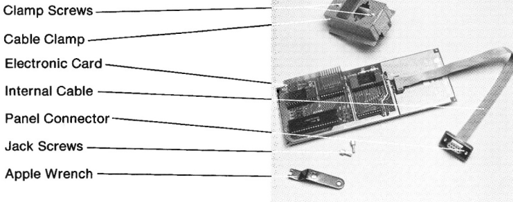
Figure 2-5. Apple II or II Plus Connector Parts
