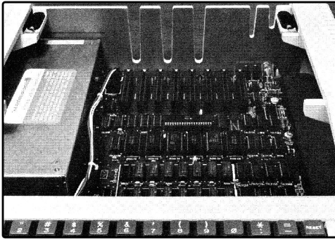
APPLE II I/O SLOTS
