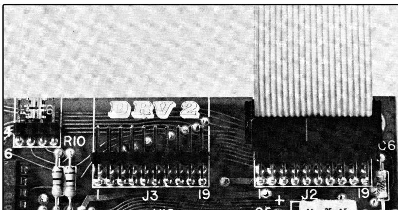
CONNECTING THE CABLE TO THE CONTROLLER
