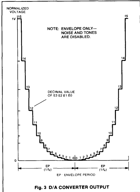
Fig. 3 D/A CONVERTER OUTPUT
