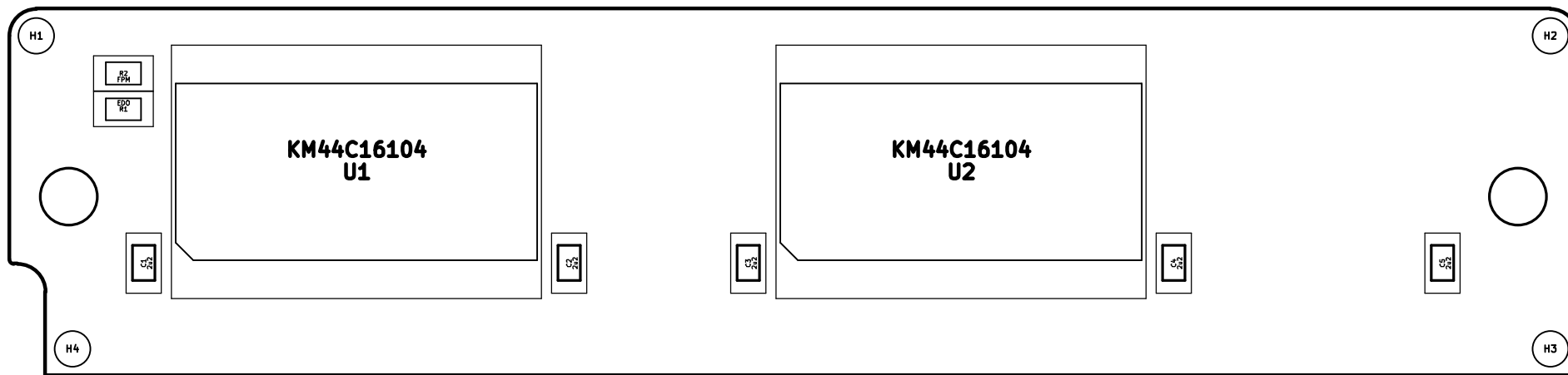
J1 DRAM-SIMM-30
