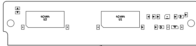
J1 DRAM-SIMM-30
