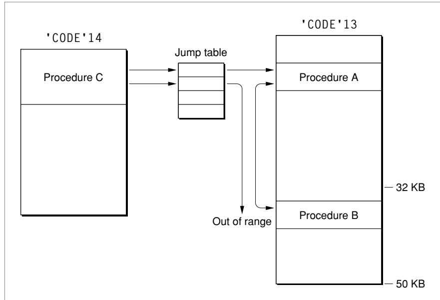
Figure 10-7 Branch islands and intersegment references
