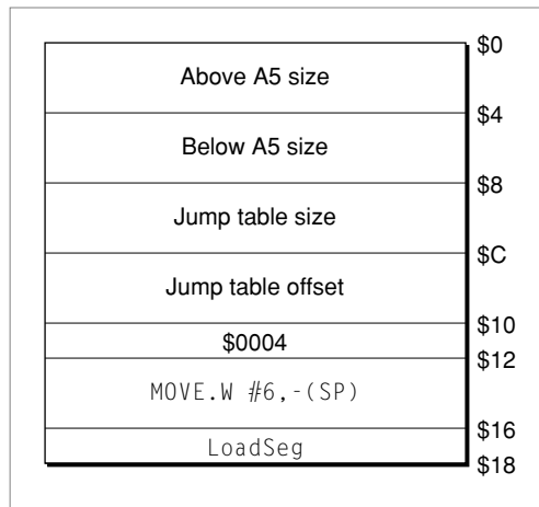
Figure 9-4 The ‘CODE’ 0 resource
